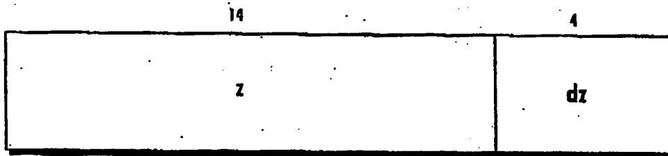
Fig. 33 DEPTH PIXEL FORMAT
